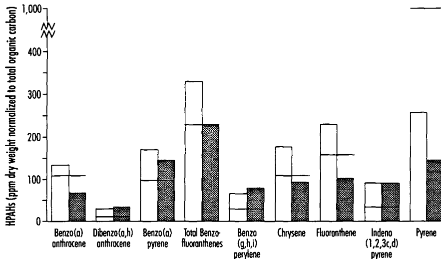
Figure 2. 1992 - 1993 concentrations of HPAH compounds at Elliott Bay, south side.
