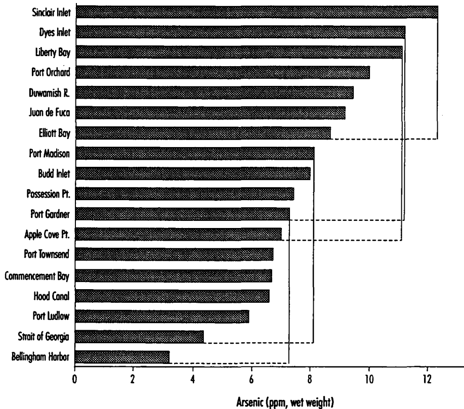
Figure 11. Arsenic in English sole muscle tissue, 1992. (Mean arsenic concentrations at sites connected by lines are not significantly different.)
