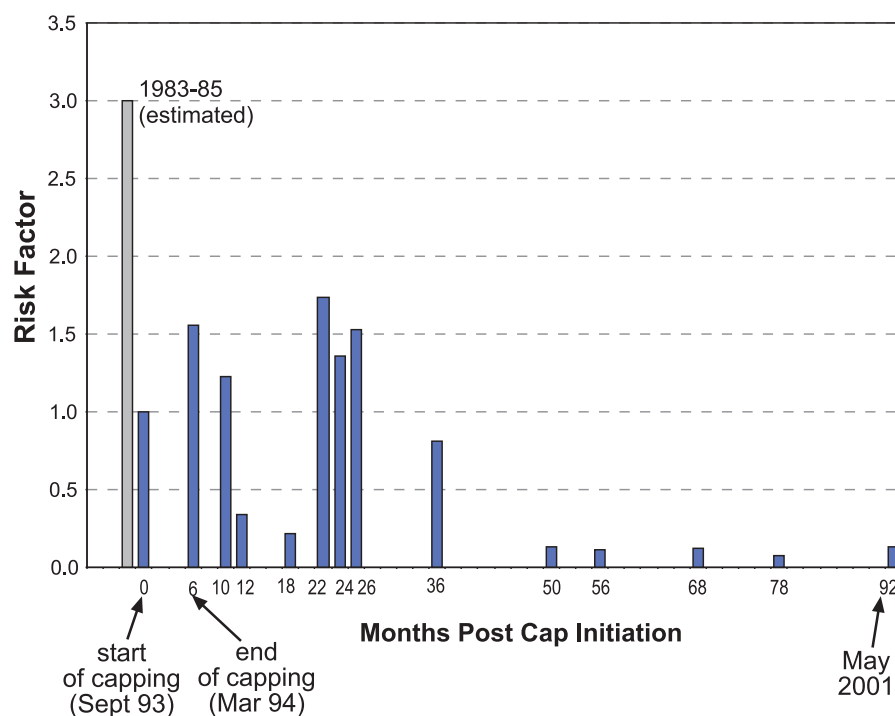
Figure 4-20. Risk of developing toxicopathic liver lesions in English sole from Eagle Harbor, prior to and following capping of contaminated sediment at this site, relative to risk at the time of capping.
