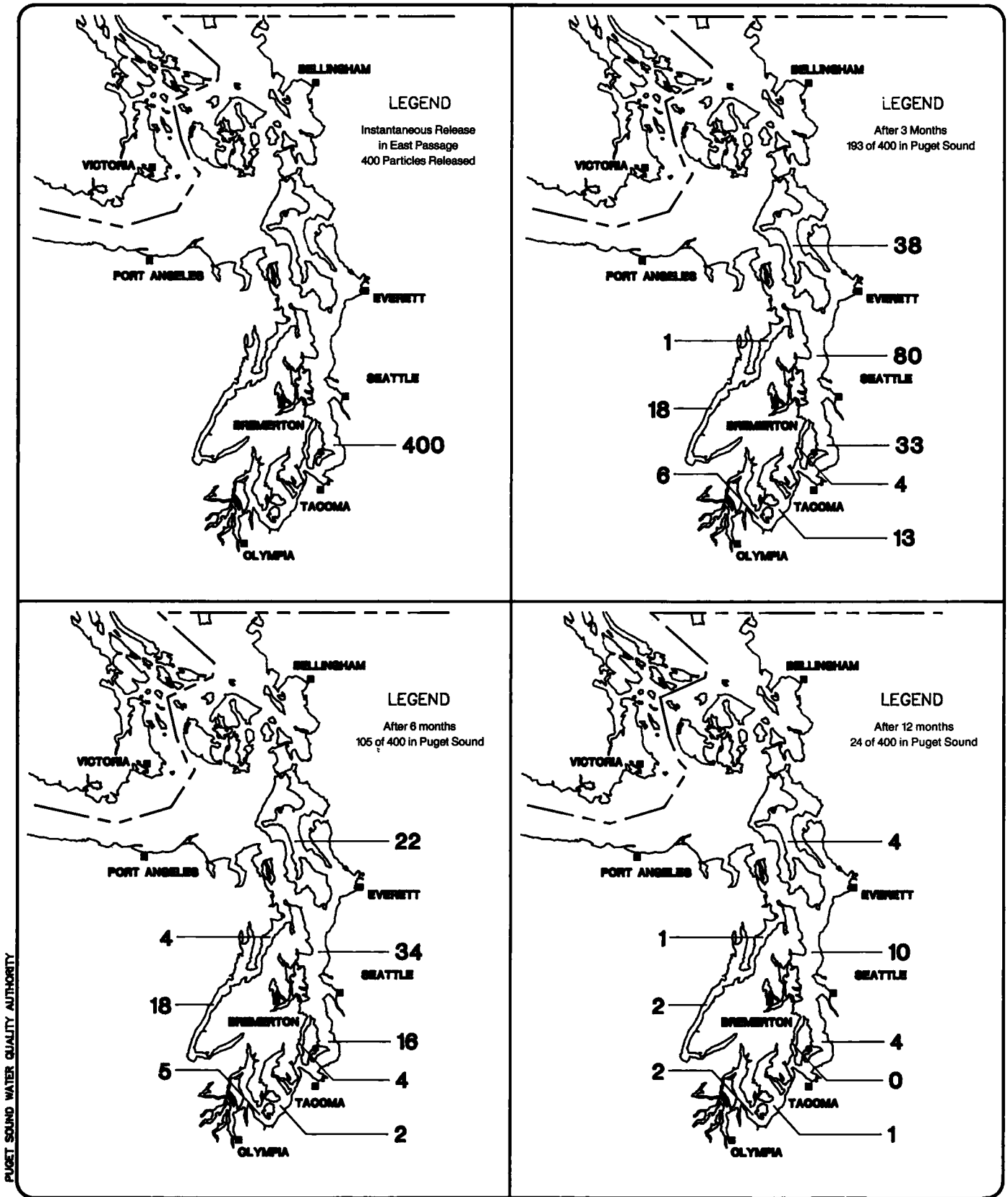
Figure 16 DISPERSION OF THEORETICAL WATER PARCELS IN PUGET SOUND
