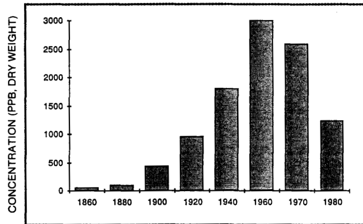
COMBUSTION PAH'S
